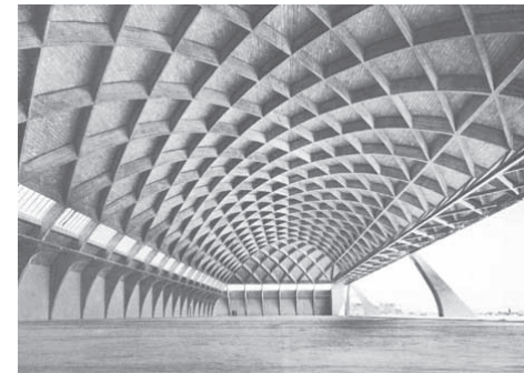
AIRPLANE HANGER - Pier Luigi Nervi (Orbetello, Italy)
